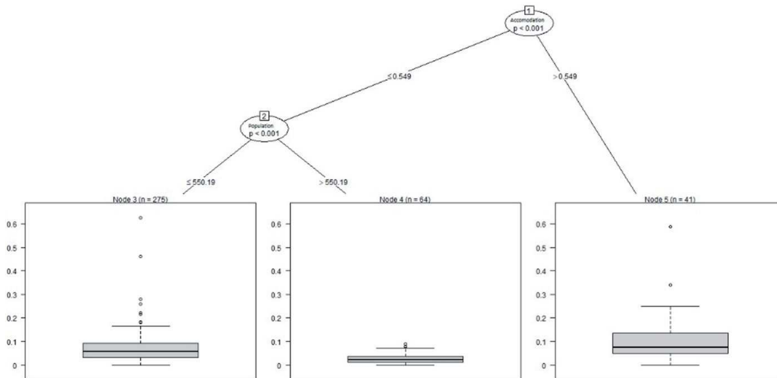
Figure 3. A regression tree model for MLR activities built with ctree algorithm
