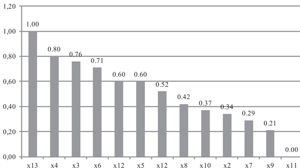
Figure 5. The significance of variables for y
