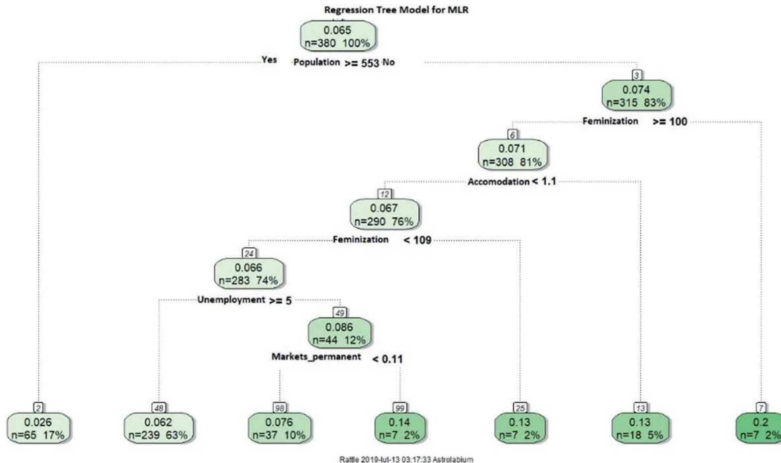
Figure 2. A regression tree model for MLR variable built with CART algorithm
